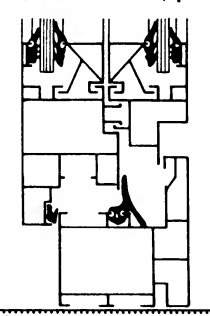
⑧ Plastic double glazed window, composite casement, in-trapane sun screen (up to 45 dB)
